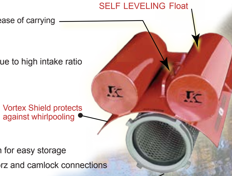
Full time swiveling strainer • FBS602 Big Water
